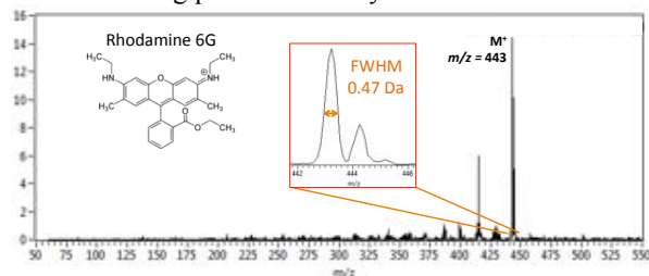
Fig. 4 Flight mass spectrometer in laser desorption/ionization mode achieves ~femtomole per mm 2 limit of detection per spectrum for a nonvolatile aromatic organic compound.
