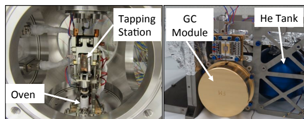
Fig. 3 The flight models of the Tapping Station (left; to seal pyrolysis ovens) and the GC subsystem (right) have been assembled and are undergoing “ultra-clean” functional tests.
