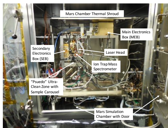
Fig. 1 Flight linear ion trap MS assembly with laser in Mars environment simulation chamber to match mechanical, thermal, pressure, and contamination level that MOMA will experience on the ExoMars rover. Configuration supports either external commercial GC, via gas feedthroughs, or flight model GC within the existing mechanical structure.
