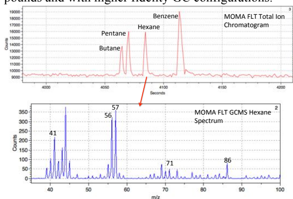
Fig. 2 Flight MOMA GCMS total ion chromatogram (top) shows nominal detection of hydrocarbons in He. The hexane GC peak is sampled with multiple EI spectra such as shown (bottom) with its characteristic fragmentation pattern.
