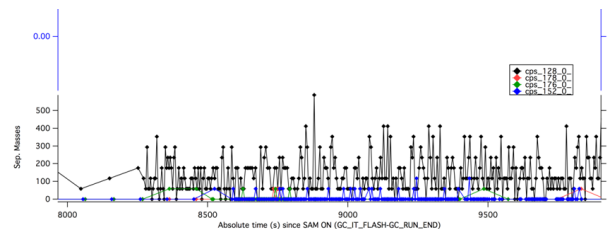
Figure 4: SS-GCMS analysis of the Rocknest soil focusing on single m/z ions related to simple 2 and 3 rings PAHs: naphthalene, anthracene and phenanthrene. No signal appears above the background level, assessing the non detection of these compounds in the gases evolved from the sample.
