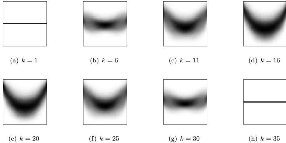
FIGURE 9. Fixed time marginals (e_{t_k})_{\#}\mu on the cone section M \times [r_{min}, r_{max}] ( r_{min} = 0.6 , r_{max} = 1.4 ) for the non-deterministic associated with the boundary conditions specified by the map in equation (8.16).
