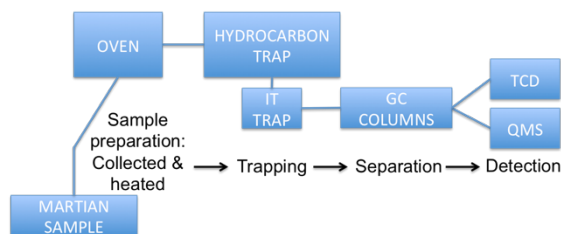
Figure 1: simplified analytical channel from sample collection to the detection and identification of the organic molecules.
