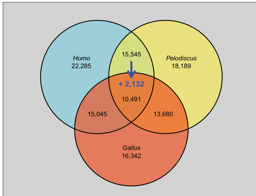
FIG. 1. Number of available annotations in human ( Homo ), Chinese soft-shell turtle ( Pelodiscus ) and chicken ( Gallus ). Numbers in intersections correspond to the amount of 1-to-1 orthologs available for each pair of species and, in blue, the total number of new sequences corresponding to orthologs missing in Gallus annotations that were recovered in at least one avian species.
