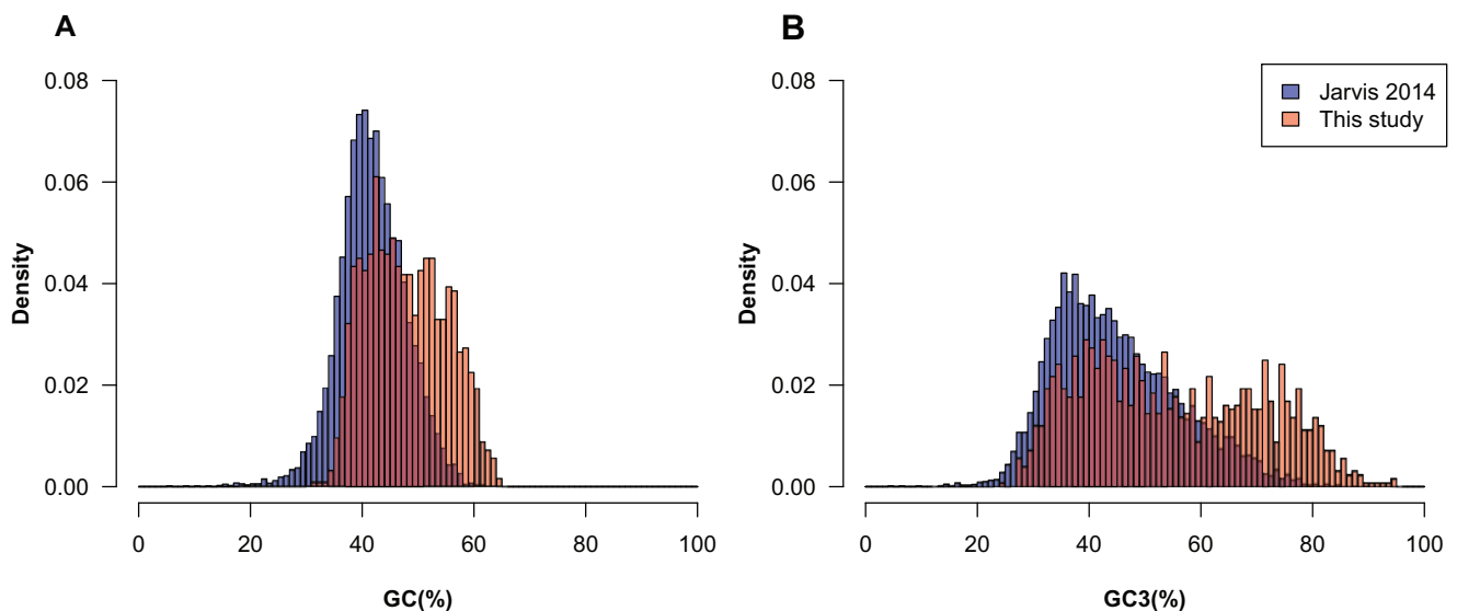
FIG. 2. Comparison of (a) GC total and (b) GC3 for the set of 8,235 genes produced in Jarvis et al (2014), in blue, and the sequences retrieved in this study, in red.
