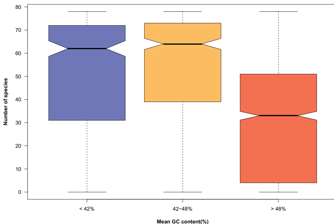
Fig. 3. Number of genes recovered as a function of GC content. Genes with high GC content (red) are less often recovered than those with low (blue) and intermediate (orange). r = -0.42 ; P < 2.26E-16 .
