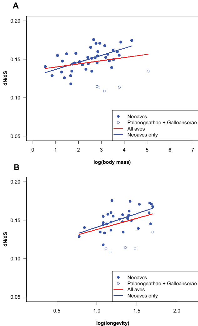
FIG. 4. Correlation between dN/dS and body mass (a) and longevity (b) in Aves. Empty dots correspond to Palaeognathae ( Struthio and Tinamou ) and Galloanserae ( Anas , Gallus , and Meleagris ). Solid dots correspond to Neoaves. Traits correspond to linear regressions for all aves in the data set (red) and Neoaves only (blue).
