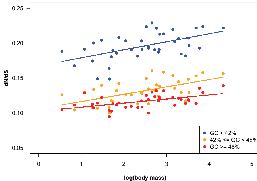
Fig. 5. Correlation between dN/dS and body mass in Neoaves, for gene sets differing in total GC content.
