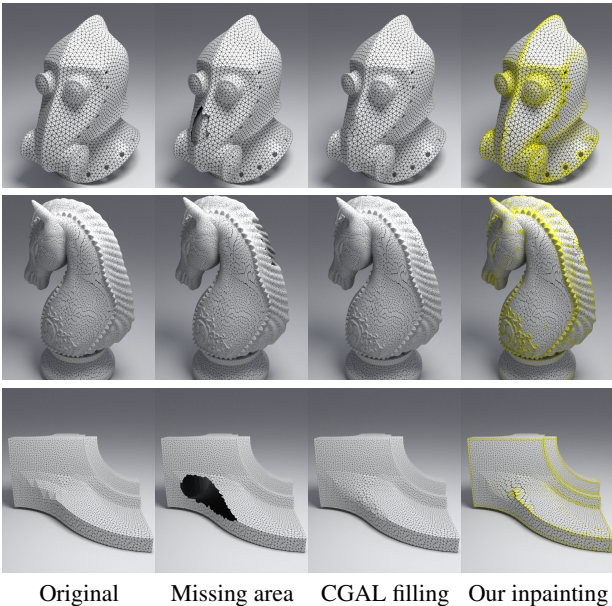
Figure 11: Inpainting results. The recovered feature field v is shown in yellow.
