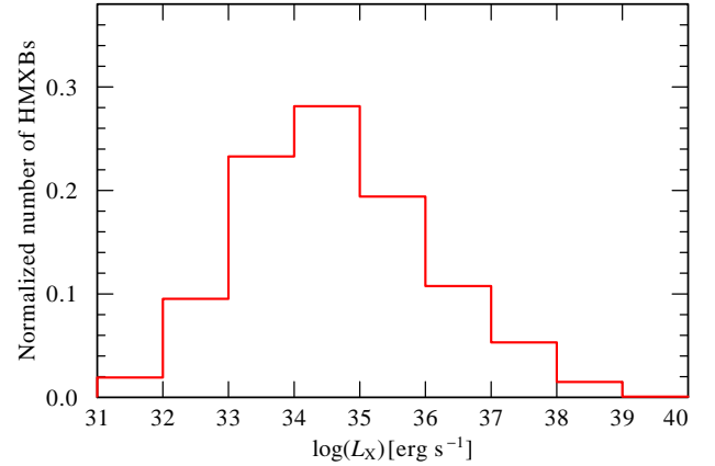
Fig. 1. Model X-ray luminosity probability distribution of wind-accreting HMXBs (see text for the model description).
