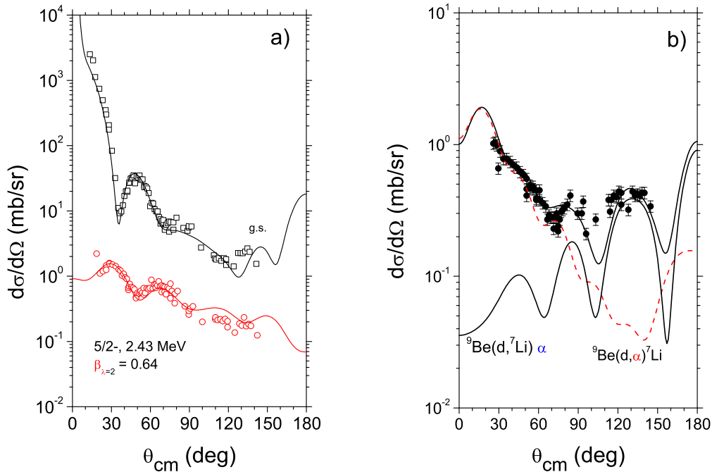
Figure 3. a) Experimental angular distribution for elastic( \square ) and inelastic scattering( \circ ) of 19.5 MeV deuterons from ^9\text{Be} target compared with the calculations. The curves are the results of the optical-model and the coupled-channel calculations. b) Experimental angular distribution ( \bullet ) for ^4\text{He} + ^7\text{Li} reaction channel (see details in text).
