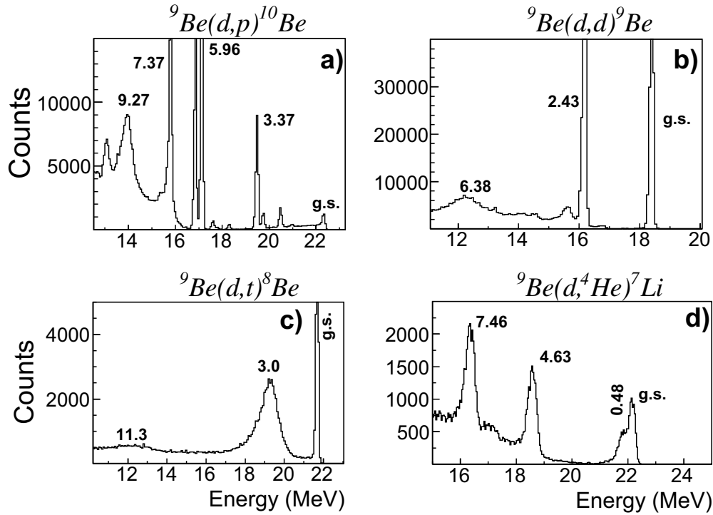
Figure 2. Total deposited energy spectra measured at \theta_{lab}=32^\circ for the detected p (panel a), d (panel b), t (panel c), and ^4\text{He} (panel d). The ground and the excited states of ^7\text{Li} for the case of detected complementary product ^4\text{He} as well as the ground states and the excited states for ^8\text{Be} , ^9\text{Be} , and ^{10}\text{Be} in the case of detected t , d , and p , as complementary products, respectively, were unambiguously identified.
