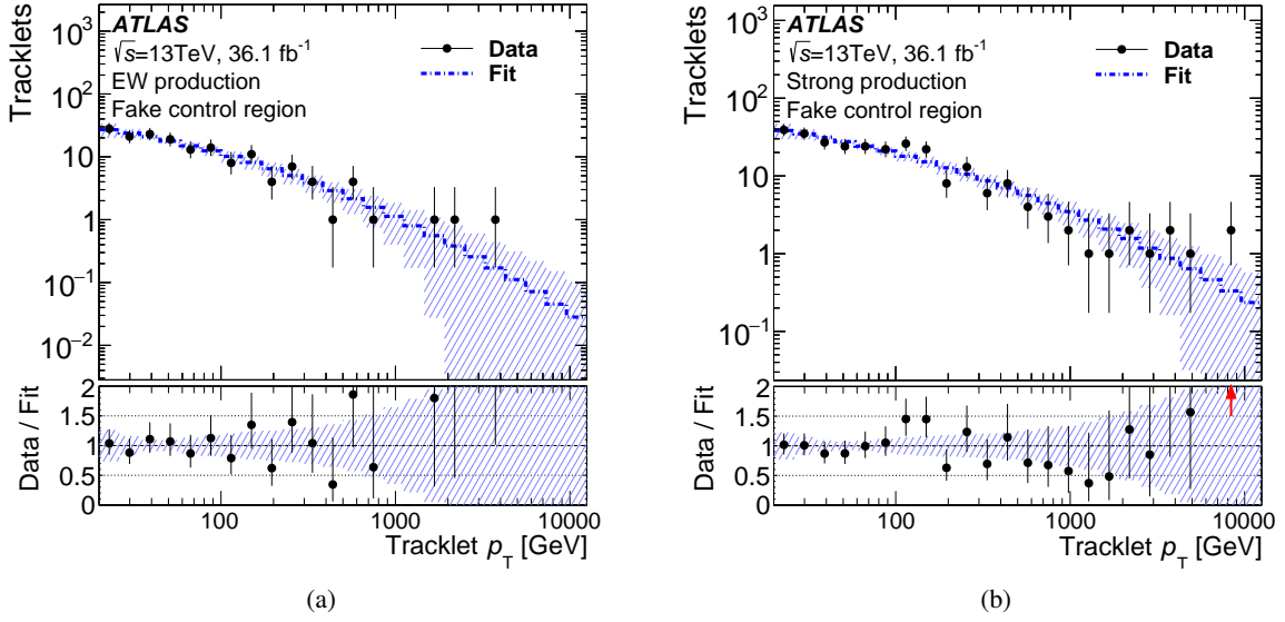
Figure 6: Fit on the fake-tracklet control sample for (a) the electroweak production channel and (b) the strong production channel. The black markers show data. The blue line and the band show the histogram made from the fit function and its uncertainty. The bottom plot shows the ratio of the observed data to the fit histogram. The chi-square per degrees of freedom of the fit are 5.4/14 and 8.5/19 for the electroweak and strong production channels respectively. Red arrows in the Data/Fit ratio indicate bins where the corresponding entry falls outside the plotted range.
