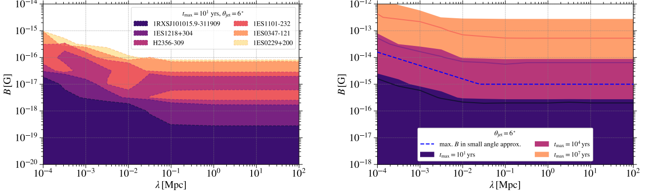
Figure 17. 95 % lower limits on the field strength of the IGMF for \theta_{\text{jet}} = 6^\circ . Left: Exclusions for t_{\max} = 10 years for individual sources. Right: Combined exclusion limits for different blazar activity times. The solid lines indicate the combined limits if the sources 1ES 0229+200 and 1ES 1218+304 are excluded from the sample. Above the blue dashed line, the small angle approximation adopted by ELMAG breaks down for an increasing number of cascade photons (cf. Eq. (8) where an energy of 1 GeV has been assumed for the cascade photons).
