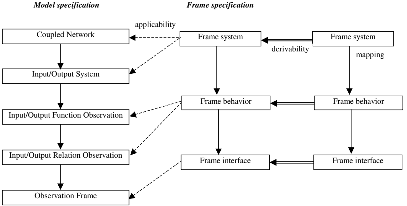
Figure 9. Specification hierarchies for models and frames, and their relationships
