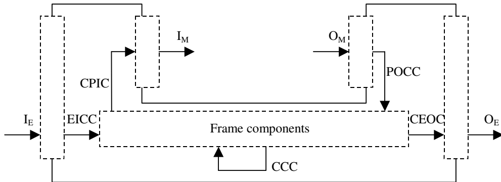
Figure 3. Frame system
