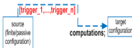
Figure 27. Transition externe de configuration
