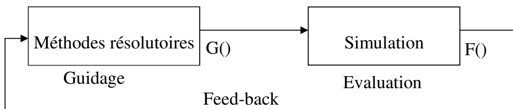
Figure 6. Couplage simulation-centré
