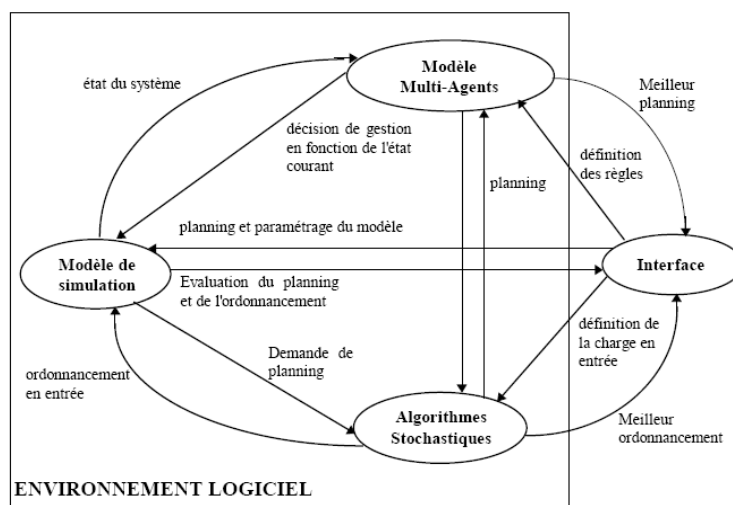
Figure 10. Couplage Triple
