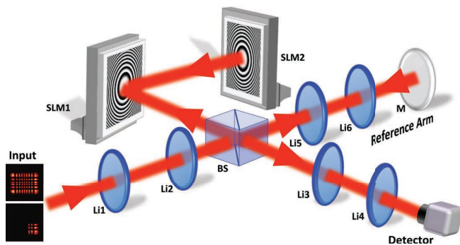
FIG. 3. Schematic of the optical set-up. For the non-interferometric measurement, only the arm of the Michelson interferometer that contains the SLMs is used. The anisotropic lenses L1 and L3 are implemented on SLM1, while L2 is implemented on SLM2. The input field is imaged onto SLM1 using a 4f system (unit magnification) formed by lenses Li1 and Li2. In the reference arm (used for the interferometric measurements), the field is relayed onto mirror M using another telescope formed by lenses Li5 and Li6 (magnification=0.5). The interference signal is relayed to the CCD detector using the 4f system formed by lenses Li3 and Li4 (magnification=0.5). Distances are not drawn to scale.
