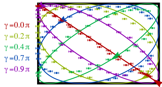
FIG. 6. Elliptic trajectories traced by the centroid given a constant PB phase determined by the values of \gamma (between 0 and 0.9\pi ). The solid curves correspond to the theoretical expectation. Error bars for centroid determination are included in both directions. The arrowheads indicate the location of zero Gouy phase and the direction of its increase.
