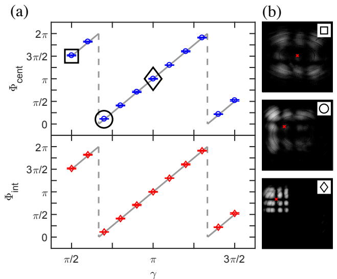
FIG. 4. PB phase measurement results. (a) Measured PB phase as a function of \gamma using the centroid of the blocked beam (circles, top panel), and interferometric measurements (diamonds, bottom panel). The non-interferometric results are wrapped onto [0, 2\pi) for comparison with the interferometric ones. Error bars are shown for both, as well as the theoretical value (gray line). (b) Measured intensity of the transformed blocked beam (plotted on a log scale) with centroids as red crosses, for different \gamma . The symbols at the insets correspond to the markers in (a).
