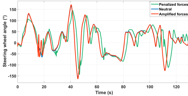
Fig. 8. Steering wheel angle in case of control allocation tuning.
