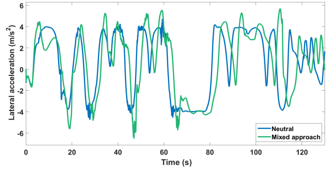
Fig. 9. Lateral acceleration in case of mixed tuning.
