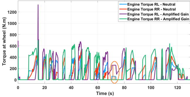
Fig. 4. Engine torques in case of reference tuning.
