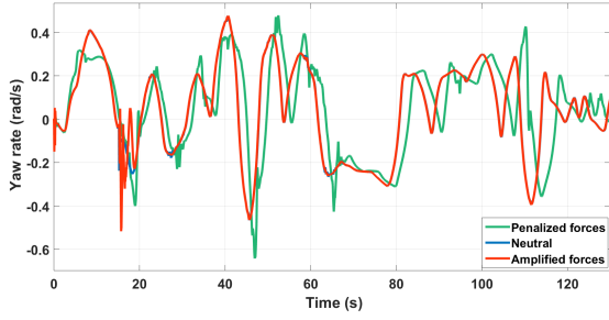
Fig. 7. Yaw rate responses in case of control allocation tuning.
