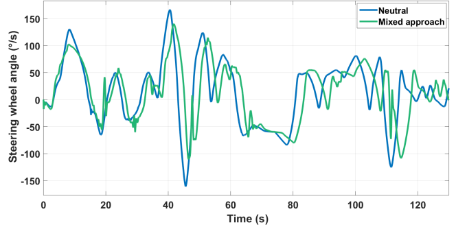
Fig. 10. Steering wheel angle in case of mixed tuning.
