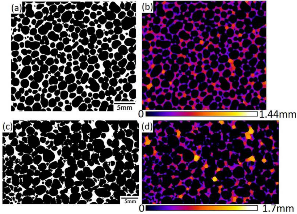
Fig. 14. (a) Binarized image and (b) the image after calculating with “Local Thickness” for solid material thickness of the MF74 (the calculated average solid material thickness \bar{t} is 0.378 mm, and the standard deviation s is 0.154 mm), (c) binarized image and (d) the image after calculating with “Local Thickness” for solid material thickness of the GI80dyn ( \bar{t} is 0.459 mm, and s is 0.256 mm).
