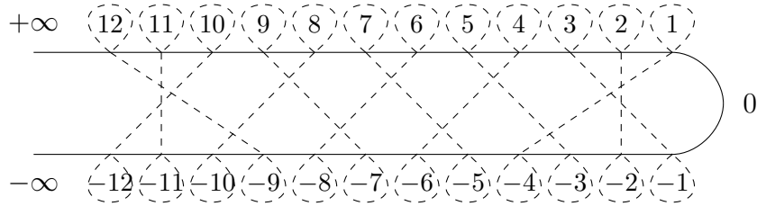
Figure 4: An illustration of the intervals in T_6 .
