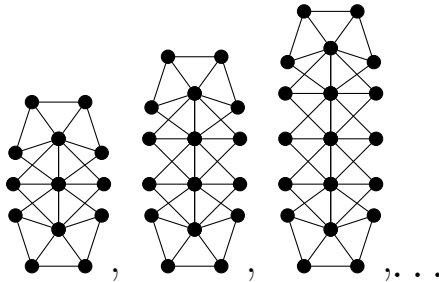
Figure 3: The infinite antichain \mathcal{A}_M of Matoušek, Nešetřil, and Thomas.
