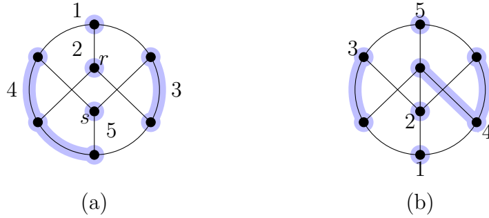
Figure 9: Models of \widehat{K}_4 in the proof of Lemma 11 . The numbers indicate which vertices of \widehat{K}_4 (following the convention of Figure 1 ) correspond to the subsets of vertices depicted in blue.
