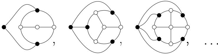
Figure 2: Thomas' alternating double wheels.
