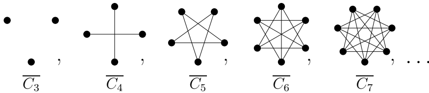
Figure 5: Antiholes antichain.
