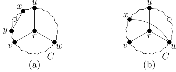
Figure 8: When C has a chord. In these examples, there is a K_4 -subdivision that does not use the white vertex, which contradicts the minimality of S . Zigzag lines depict paths with at least one edge.
