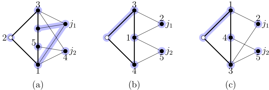
Figure 11: Induced minor-minimal counterexamples in the proof Lemma 23 contain the Gem as induced minor. The vertex c is depicted in white. The numbers indicate which vertices of the Gem (following the convention of Figure 1 ) correspond to the subsets of vertices depicted in blue.
