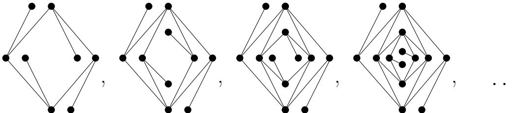
Figure 6: Nested lozenges.
