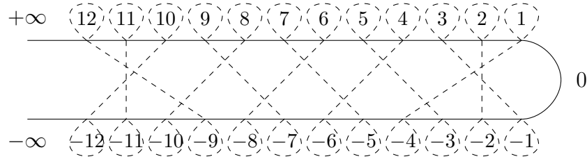
Figure 4: An illustration of the intervals in T_6 .
