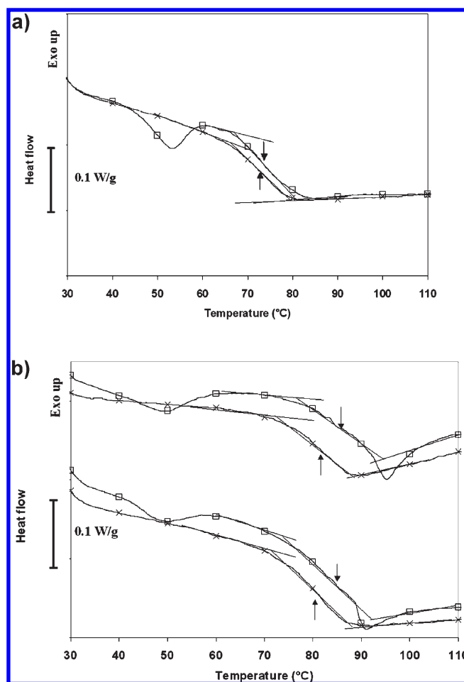
Figure 7. DSC thermogram with two successive scans (1st, \square ; 2nd, \times ) for the nondeformed sample (a) and the two deformed samples (b) at 90 °C (top) and 115 °C (bottom). The arrows indicate the glass transition.
