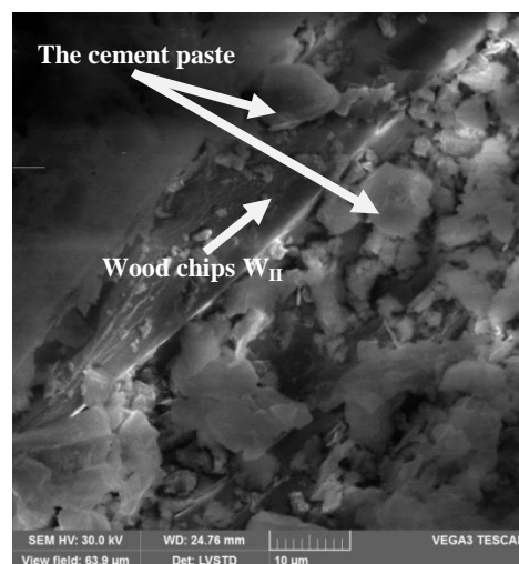
Figure 5: Microstructural observation (with SEM) of wood chips treated with cement Paste.
