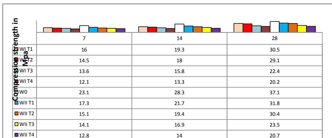
Figure 14: Compressive strength in MPa for treated wood chips based concrete at 7, 14 and 28 days.
