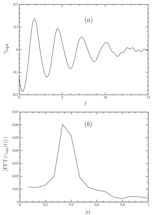
Fig. 10. Optimized control function \gamma_{\text{opt}} : (a) time evolution signal and (b) amplitude of the corresponding FFT.
