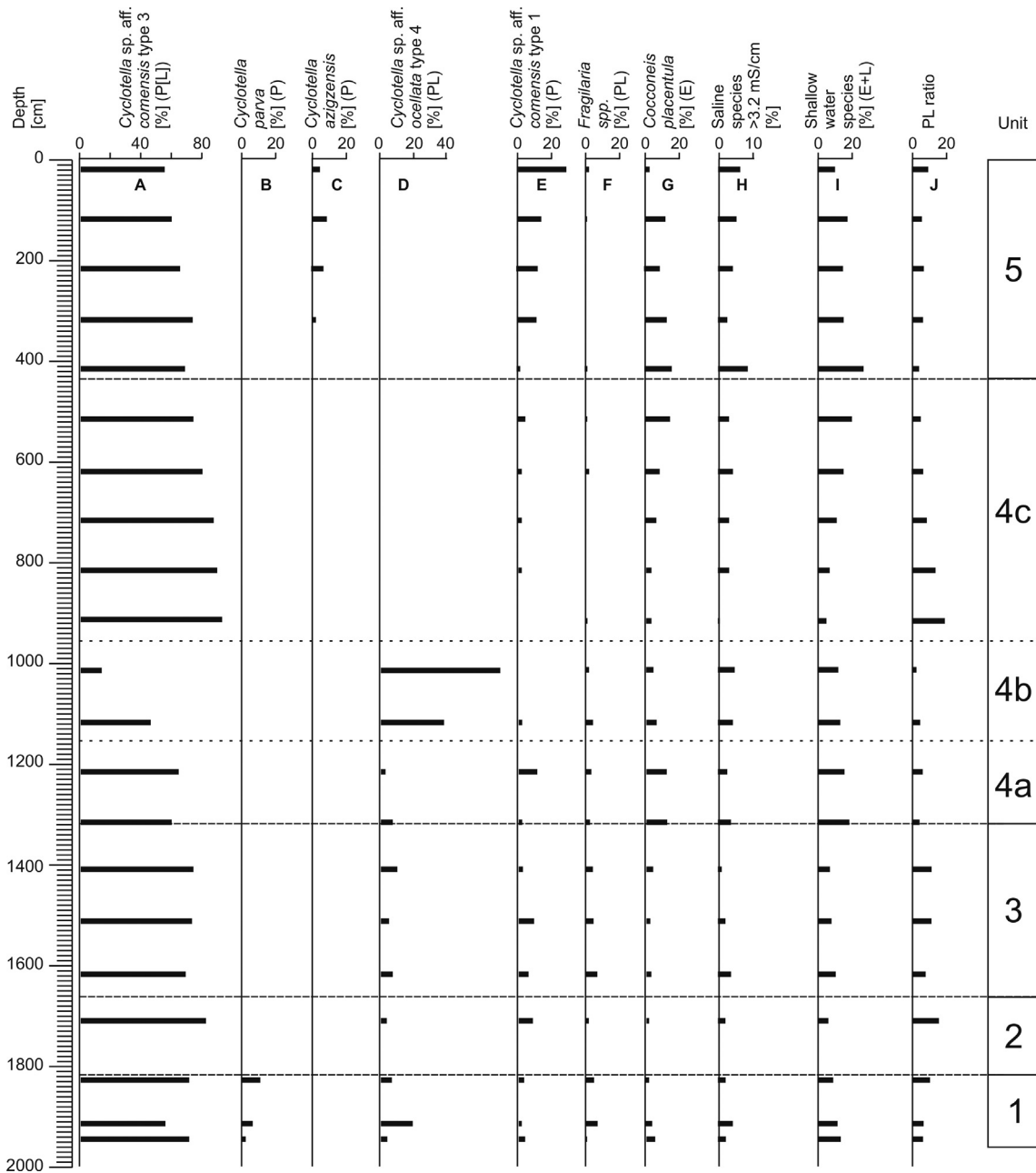
Fig. 7. First set of Sidi Ali diatom data: a) Planktonic Cyclotella sp. aff. comensis type 3, b) Planktonic Cyclotella parva , c) Planktonic Cyclotella azigzensis , d) Planktonic and littoral Cyclotella sp. aff. ocellata type 4, e) Planktonic Cyclotella sp. aff. comensis type 1, f) Planktonic and littoral Fragilaria spp. g) Epiphytic Cocconeis placentula , h) Epiphytic and littoral saline species, i) Epiphytic and littoral shallow water species, j) Planktonic/Littoral diatom ratio.
