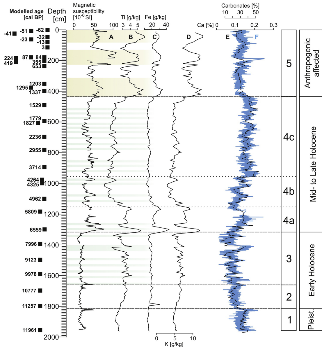
Fig. 5. Sidi Ali palaeomagnetic and silici-clastic proxies: a) volume magnetic susceptibility; b) XRF Ti content; c) XRF Fe content; d) XRF K content; e) carbonate content and f) calibrated Ca XRF scanning data. Blue bars indicate internal variability of magnetic susceptibility peaks, which are coeval with carbonate peaks (Fig. 8e) and TOC troughs (Fig. 8f). (For interpretation of the references to colour in this figure legend, the reader is referred to the web version of this article.)
