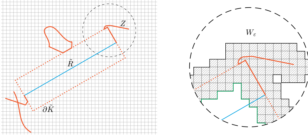
Figure 6: On the left we represent the finer grid for the third projection step. In orange we draw the set Z := (\text{supp } \tilde{R} \setminus \text{Int } \tilde{K}) \cup \partial\tilde{K} , in particular the dotted part is \partial\tilde{K} . In the right we show a detail of the drawing with the set W_\varepsilon . The set W_\varepsilon is highlighted in striped gray and the set \partial W_\varepsilon \cap \tilde{K} in dark green.
