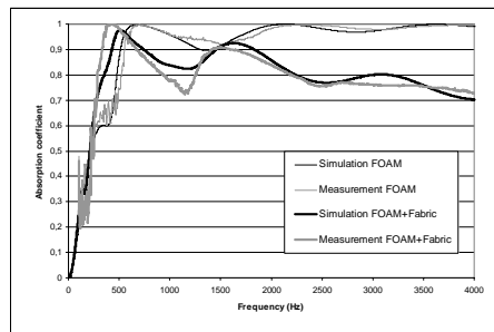
Fig 1. confrontation simulation/measurements (S configuration)
