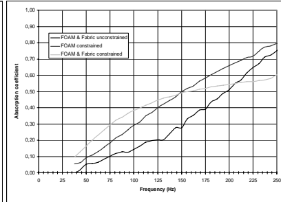
Fig 2.2. Lateral mounting conditions (measurement)
