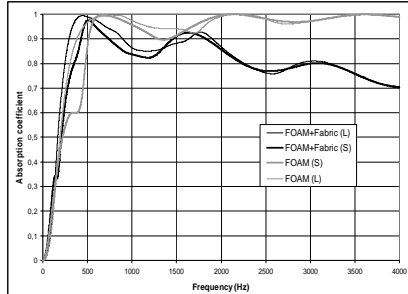
Fig 2.1. Background mounting conditions L&S (simulation)
