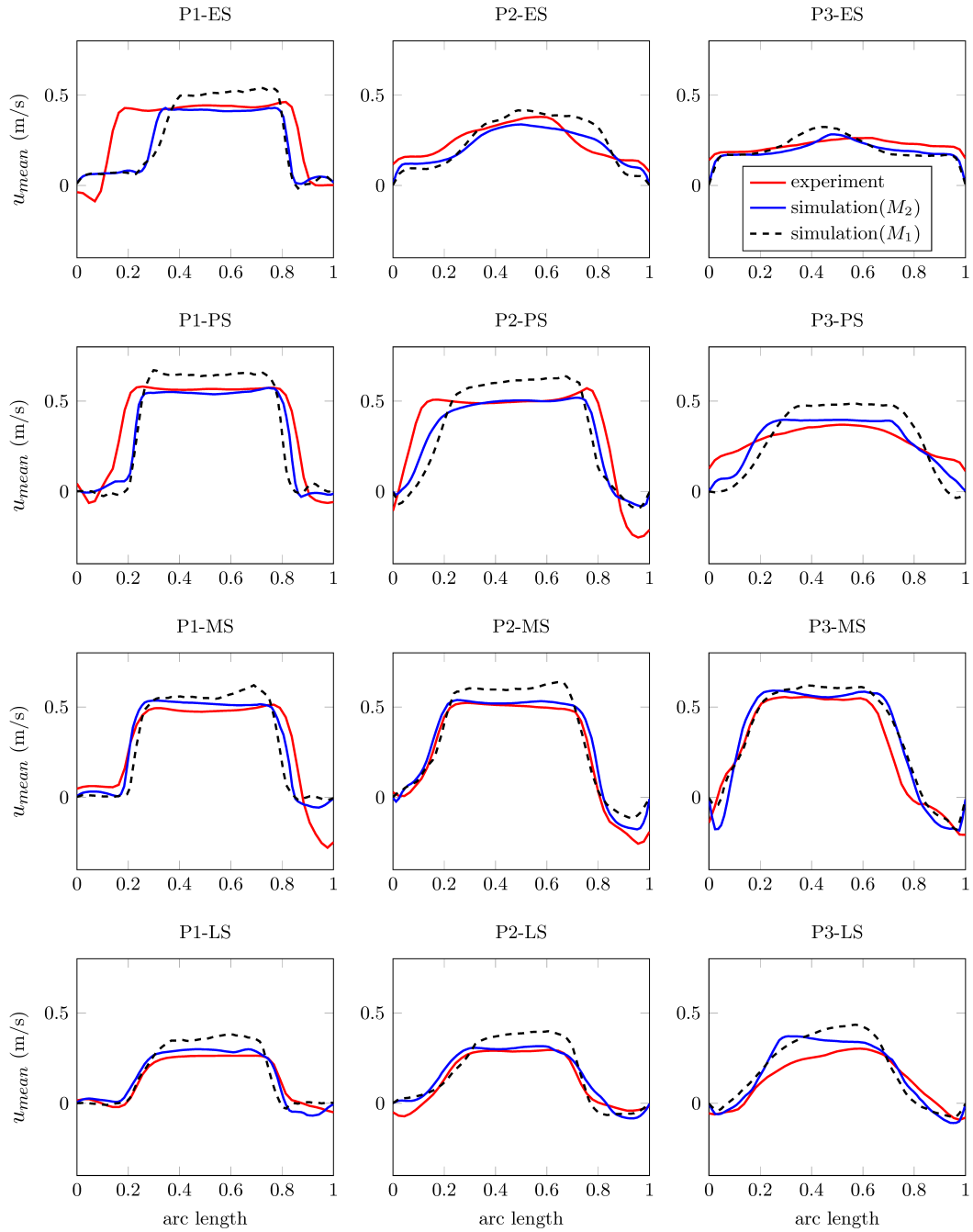
Figure 9. Comparison of the experiment (red) and the simulations for meshes M_1 (black) and M_2 (blue), for 3 successive phase-averaged velocity profiles downstream of the valve. Four different instants of the cardiac cycle are depicted (ES, PS, MS and LS).
