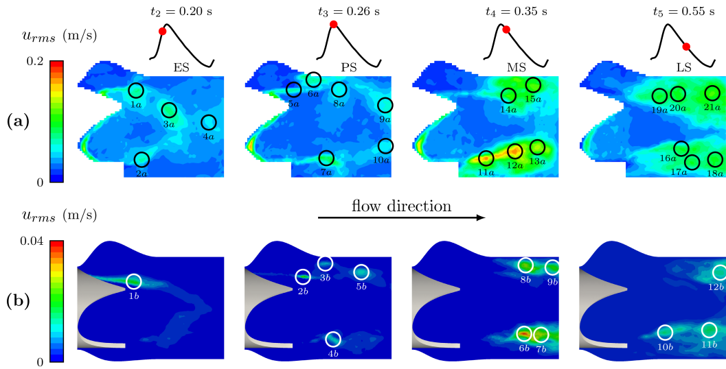
Figure 8. (a) Fields of streamwise RMS velocity obtained from the experiment. (b) Fields of streamwise RMS velocity obtained from the simulation for the fine mesh M_2 . Four different instants of the cardiac cycle are depicted (ES, PS, MS and LS).
