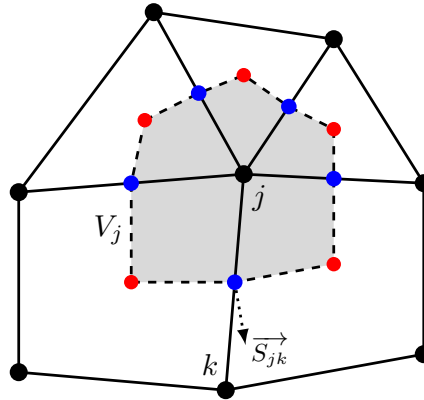
Figure 12. Dual volume V_j created around the node j of an unstructured hybrid mesh by linking the centroids of the neighboring elements (red dots) and the centers of the edges containing node j (blue dots).
