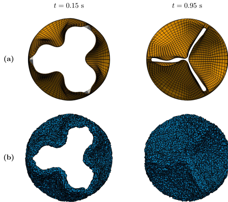
Figure 11. (a) Deformation of the valve at two different instants of the cardiac cycle ( t = 0.15 \text{ s} when the valve is opening, and t = 0.95 \text{ s} when the valve is fully closed). (b) Patch of fluid elements on which the mechanical force is regularized, illustrating how the valve is seen by the fluid.
