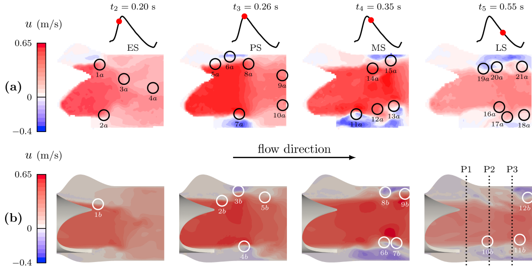
Figure 7. (a) Fields of instantaneous streamwise velocity obtained from the experiment. (b) Fields of instantaneous streamwise velocity obtained from the simulation for the fine mesh M_2 . Four different instants of the cardiac cycle are depicted (ES, PS, MS and LS).
