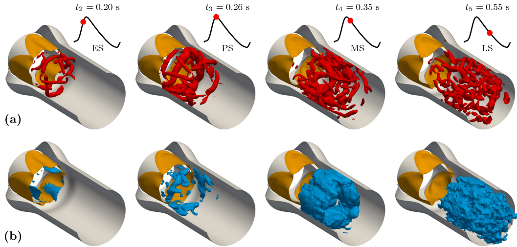
Figure 10. (a) Iso-surfaces of the instantaneous Q-criterion for the iso-value of 5000 \text{ s}^{-2} . (b) Iso-surfaces of the fluctuating kinetic energy for the iso-value of 0.08 \text{ J.m}^{-3} . Four different instants of the cardiac cycle are depicted (ES, PS, MS and LS).
