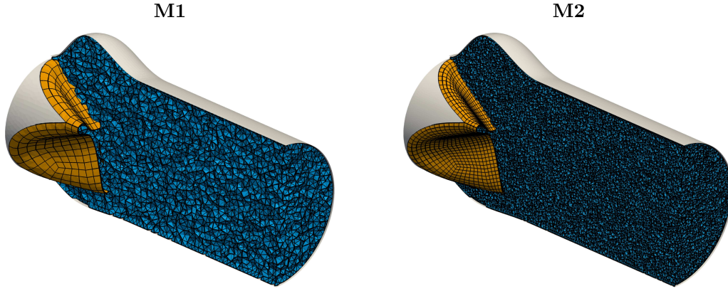
Figure 3. Computational zone of interest composed of the valve solid mesh and the aortic fluid mesh. Two levels of mesh are considered, the coarse mesh M_1 and the fine mesh M_2 .
