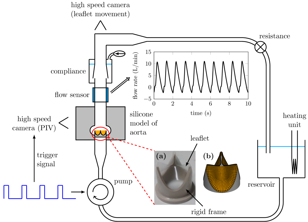
Figure 1. In-vitro pulse duplicator designed to reproduce physiological flow conditions.
