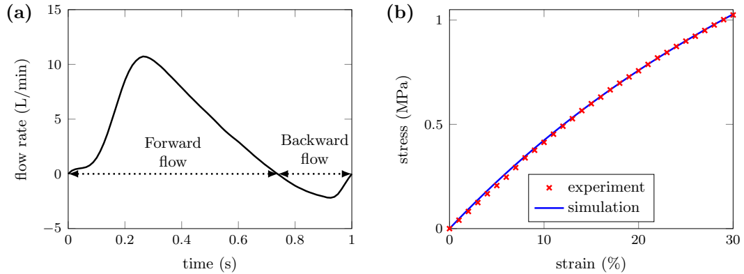
Figure 2. (a) One typical cycle of the flow rate signal measured during the experiment, used as inlet boundary condition of the simulation. (b) Stress-strain relationship extracted from the uniaxial tensile test. The material parameters G and K are determined by fitting the simulation with the experiment.
