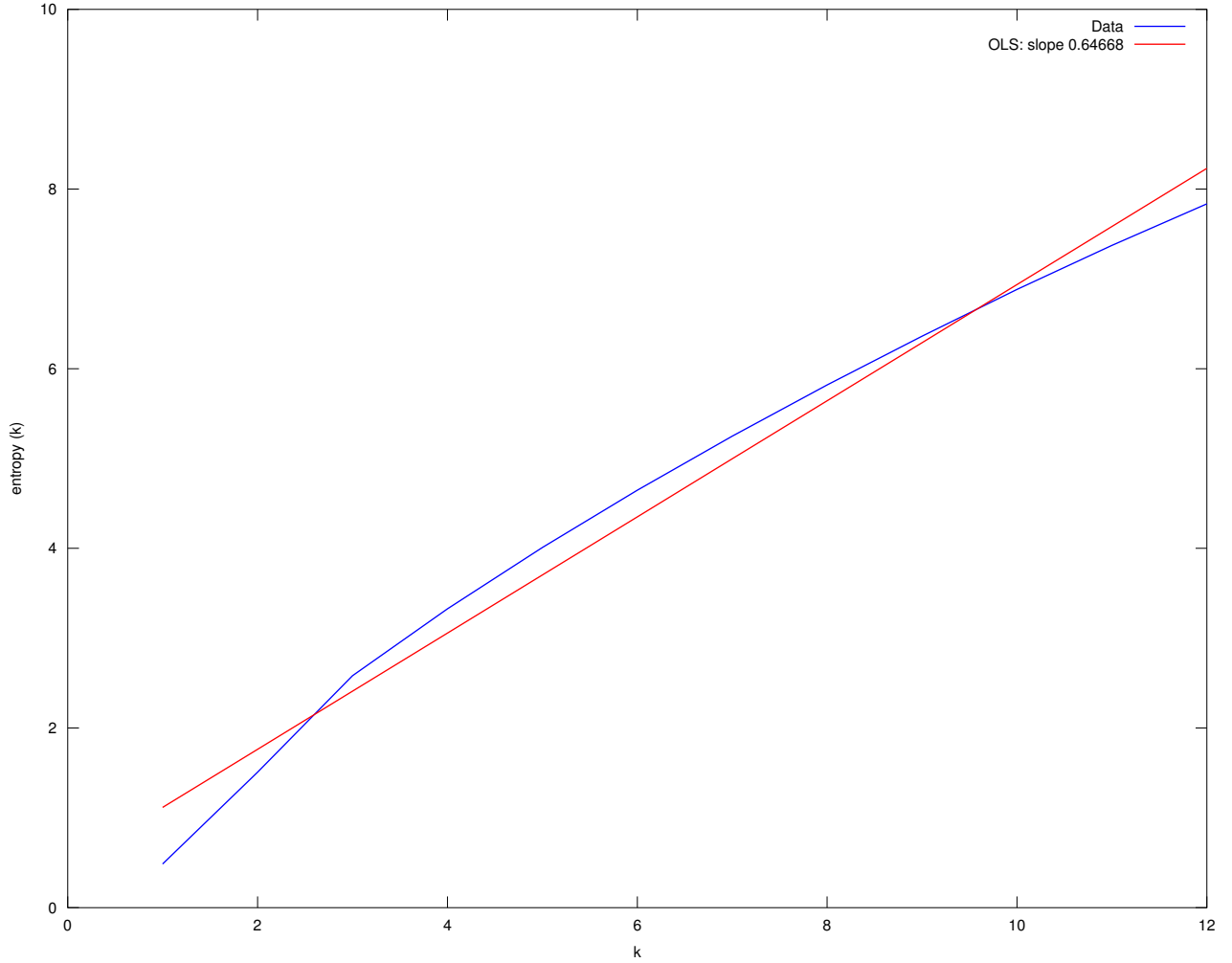
Entropy with tau = 1
