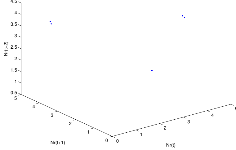
FIGURE 6. 3d plot of (N_r(t), N_r(t+1), N_r(t+2)) , with t \in \mathbb{N} , 95\,000 \leq t \leq 100\,000 for setting SP_1 .
