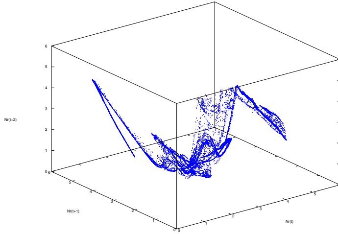
FIGURE 4. 3d plot of (N_r(t), N_r(t+1), N_r(t+2)) with t \in \mathbb{N} , 280\,000 \leq t \leq 300\,000 for setting SP.
