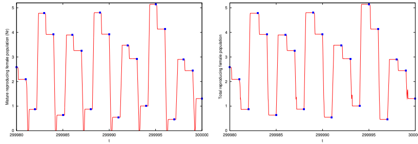
FIGURE 2. Setting SP, continuous time dynamics of reproducing female population over 20 years: mature ( N_r , left) and total population (right).
