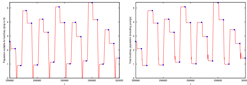
FIGURE 3. Setting SP, continuous time dynamics of butchery population over 20 years: “mature” ( \propto S , left) and total population (right).
