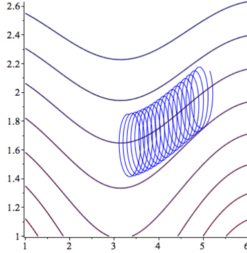
FIGURE 1. Motion of a classical particle in a strong magnetic field. The particle oscillates around a level line of B . Here B(q_1, q_2) = 2 - \cos(q_1) + q_2^2 .
