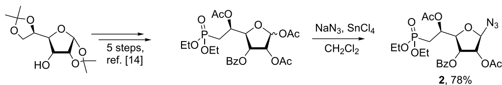
Scheme 1: Synthesis of (1-azido-2,5-di-O-acetyl-3-O-benzoyl-6-deoxy-6-diethylphosphono)- \beta -ribo-(5S)-hexofuranose 2 from commercially available diacetone D-allofuranose [15].
