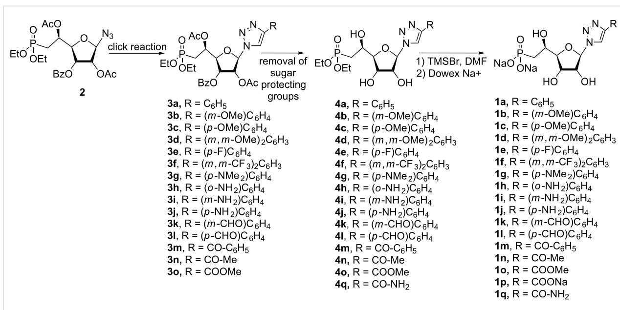
Scheme 2: General synthetic pathway for the 1,2,3-triazolo-β-hydroxyphosphonate derivatives.
