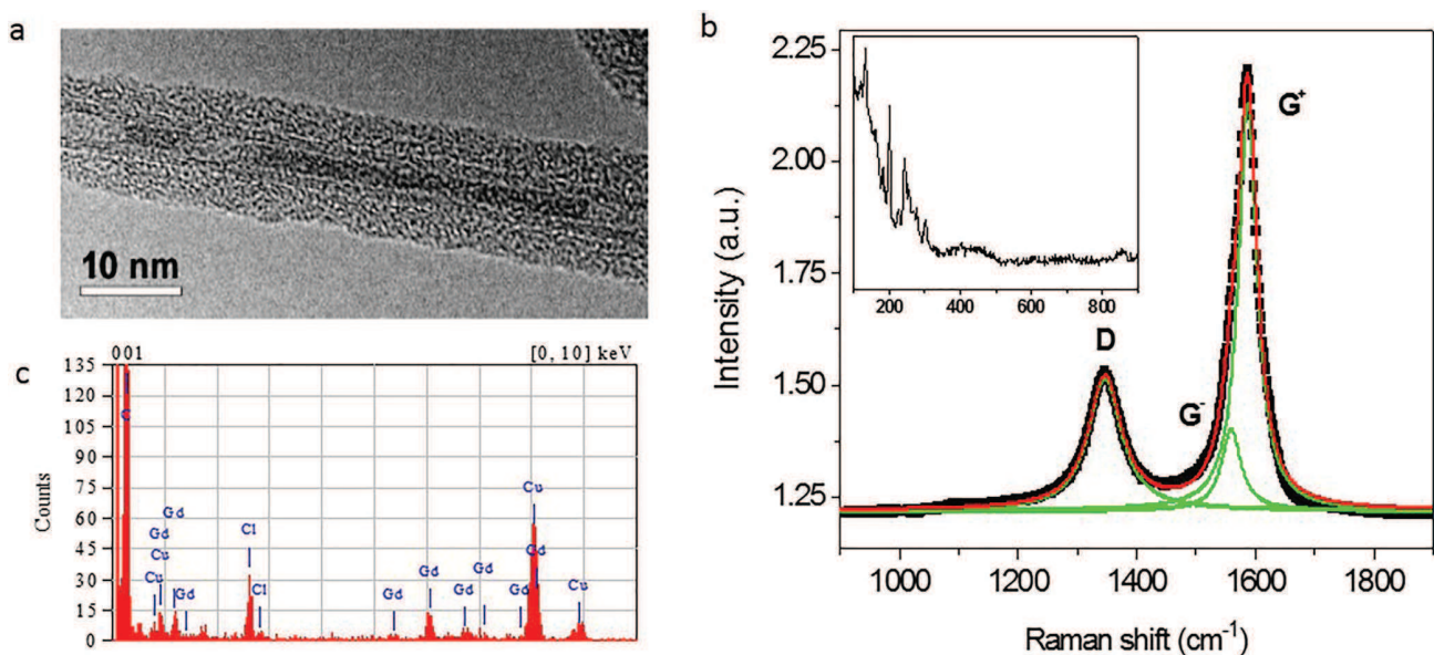
FIG. 1. (a) HRTEM image of GdCl 3 @MWNTs showing rod like structures inside the innermost tube; (b) the Raman spectrum of the GdCl 3 @MWNT, as can be seen the samples exhibits spectrum for low disordered CNT with pronounced G band and small I D /I G ratio. Convolution shows the G band can be split into two sub peaks. Inset shows multiple low wave number peak uncharacteristic of pristine MWNT. (c) EDX analysis corresponding to the boxed area in the HRTEM image showing the presence of Gd and Cl in the sample.
