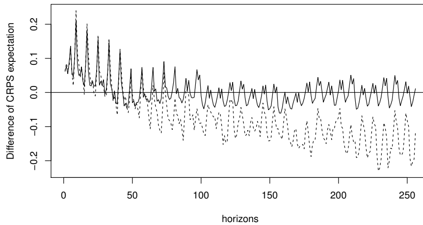
Fig. 1 Comparison of EMOS and our method CRPS expectation with that of raw ensemble The empty line corresponds to our method and the dashed one to the EMOS
