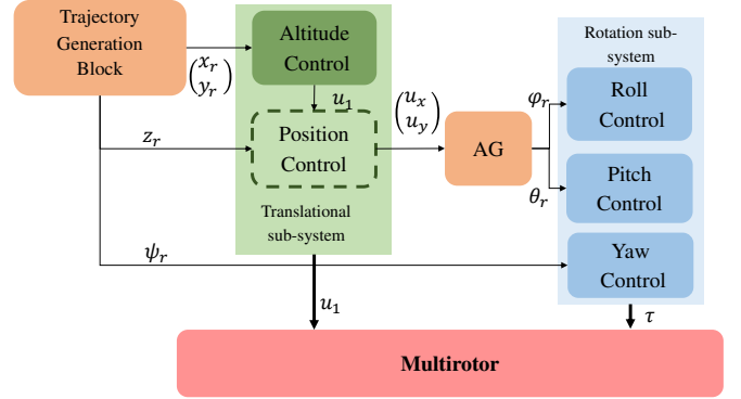
Fig. 6: Control architecture.
