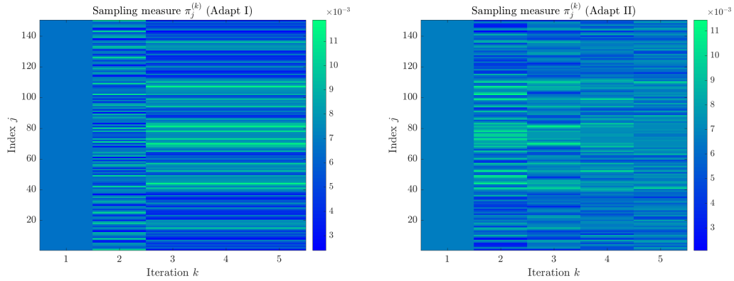
Figure 7. Evolution of the sampling measure \pi^{(k)} as a function of the iteration k for adaptive strategies (Adapt I) and (Adapt II).
