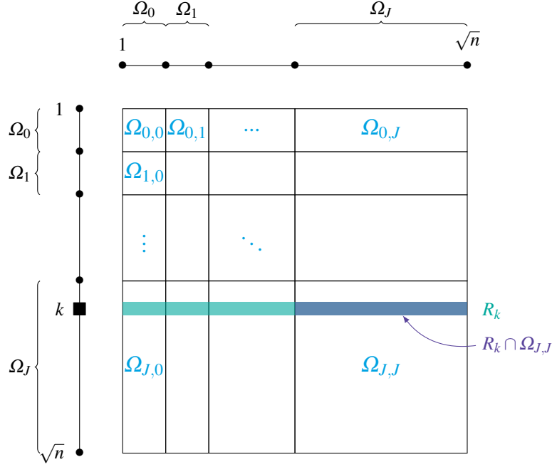
Figure 4. 2D view of the signal x \in \mathbb{C}^n to reconstruct. The vector x can be reshaped into a \sqrt{n} \times \sqrt{n} matrix. The indices can be partitioned according to the sets \Omega_{j,j'} = \Omega_j \times \Omega_{j'} for 0 \leq j, j' \leq J . R_k represents the coefficient indices corresponding to the k -th horizontal row.
