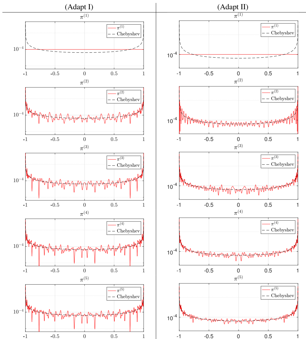
Figure 8. Convergence of the adapted measure \pi^{(k)} to the Chebyshev measure for (Adapt I), on the left column, and for (Adapt II), on the right column.
