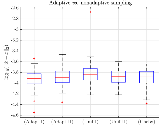
Figure 6. Approximation of f using adaptive strategies (Adapt I), (Adapt II) and nonadaptive strategies (Unif I), (Unif II), and (Cheby).
