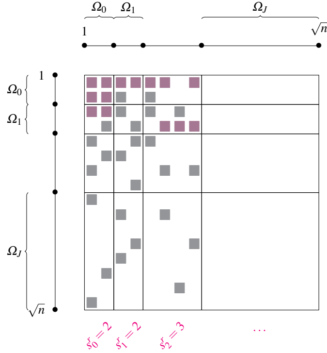
Figure 5. Example of a signal x \in \mathbb{C}^n with support denoted by squares in grey for the first vertical subbands. The quantities (s_j^r)_j are the maximal degrees of sparsity restricted to rows and respectively to vertical subbands \cup_j \Omega_{j,j} . In the Figure, they are reached for support locations highlighted in red.
