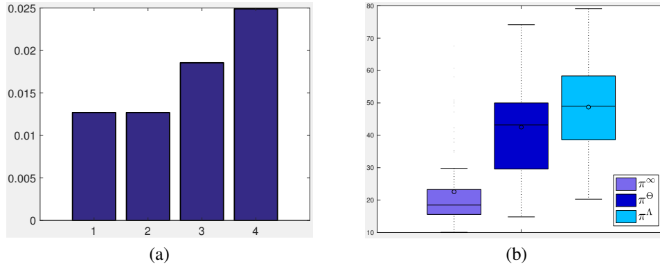
Figure 3. Boxplot of reconstruction PSNR in (b) of 100 random signals of length n = 2048 having a structured sparsity in the wavelet decomposition as in (a) ( s/n = 6\% ) from 25% measurements drawn according to \pi^\infty , \pi^\Theta and \pi^\Lambda as in Figure 2 (a,b,c). In (a), we represent the sparsity in levels structure of the randomly generated signals. The plot represents the percentage of nonzero coefficients for each subband.
