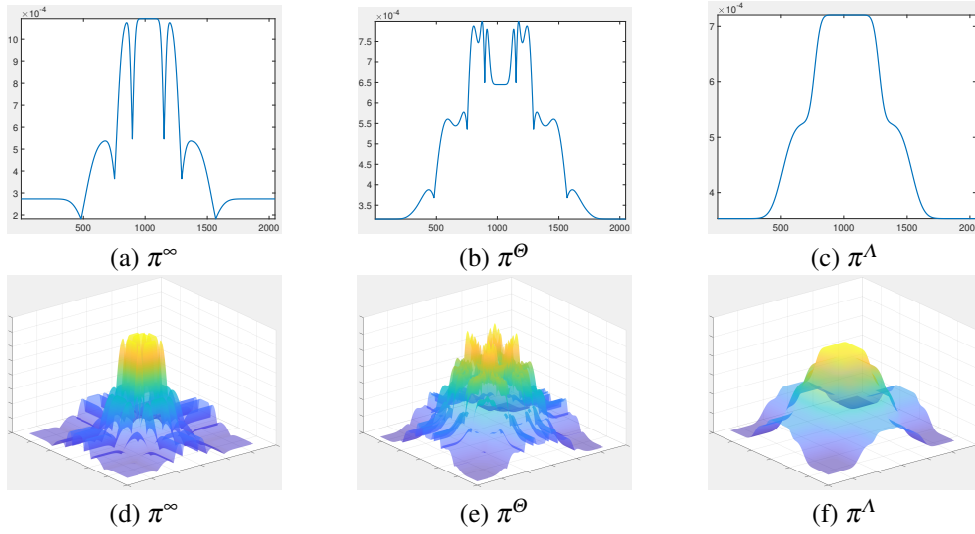
Figure 2. Comparison between sampling probability distributions chosen according to different strategies: in (a,b,c) for 1D signals with structured sparsity described in Figure 3(a), in (d,e,f) for 2D signals with the corresponding tensorized structured sparsity. In (a) and (d), the sampling probability distribution \pi^\infty is optimized to minimize the global coherence, i.e. \pi_k \propto \|a_k\|_\infty^2 ; in (b) and (e), the sampling probability distribution \pi^\Theta is optimized to minimize an upper bound to \Theta(S, \pi) , i.e. \pi_k \propto \|a_k\|_\infty \sum_{j=0}^J s_j \|a_{k, \Omega_j}\|_\infty ; in (c) and (f), the sampling probability distribution \pi^\Lambda is optimized to minimize an upper bound to \Lambda(S, \pi) , i.e. \pi_k \propto \sum_{j=0}^J \|a_k\|_\infty \|a_{k, \Omega_j}\|_\infty^2 ; the probability distributions in (d), (e), and (f) are constructed accordingly in the 2D case.
