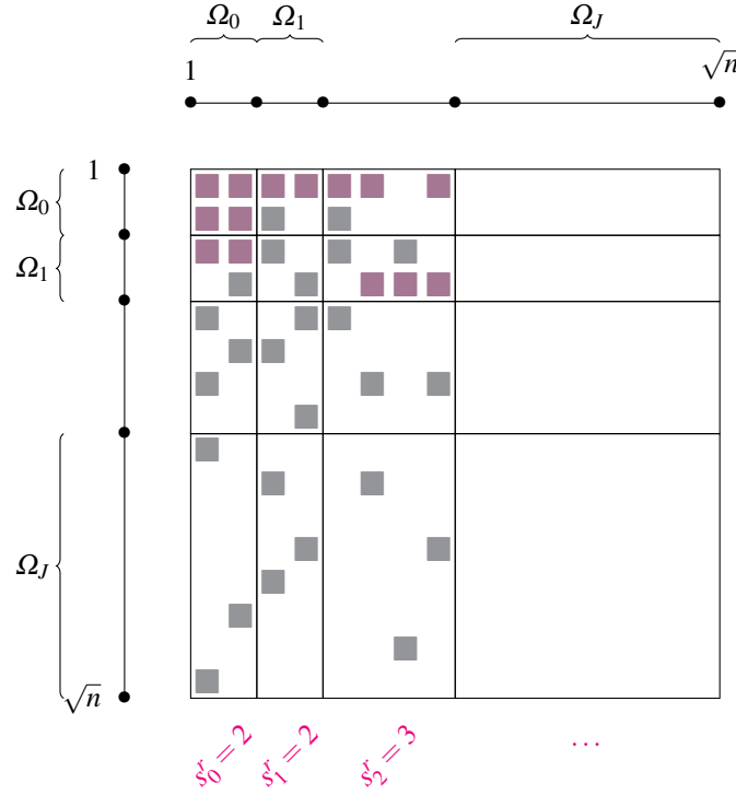
Figure 5. Example of a signal x \in \mathbb{C}^n with support denoted by squares in grey for the first vertical subbands. The quantities (s_j^r)_j are the maximal degrees of sparsity restricted to rows and respectively to vertical subbands \cup_j \Omega_{j,j} . In the Figure, they are reached for support locations highlighted in red.
