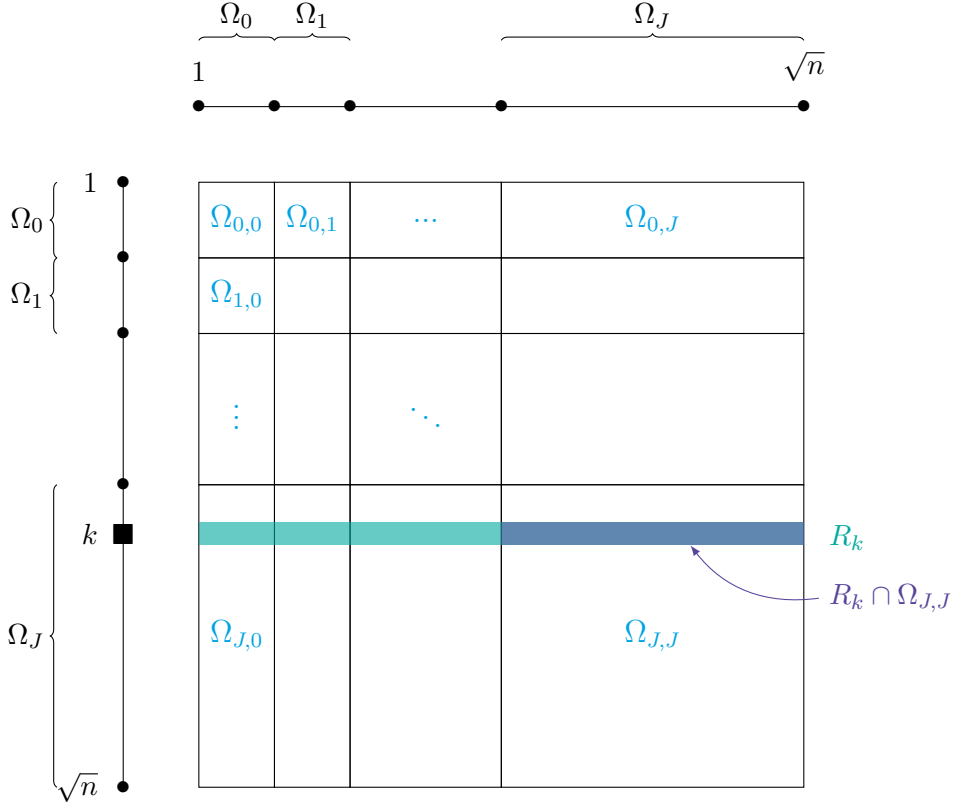
Figure 4: 2D view of the signal x \in \mathbb{C}^n to reconstruct. The vector x can be reshaped into a \sqrt{n} \times \sqrt{n} matrix. The indexes can be partitioned according to the sets \Omega_{j,j'} = \Omega_j \times \Omega_{j'} for 0 \leq j, j' \leq J . R_k represents the coefficient indexes corresponding to the k -th horizontal row.
