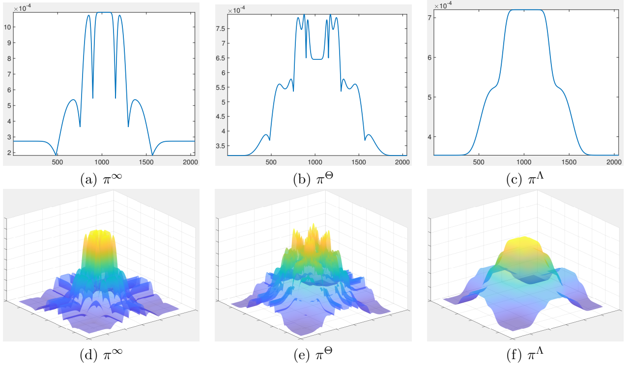
Figure 2: Comparison between sampling probabilities chosen according to different strategies for 1D signals (a,b,c) or 2D signals (d,e,f), that are sparse in levels. In (a) and (d), the sampling probability \pi^\infty is optimized to minimize the global coherence, i.e. \pi_k \propto \|a_k\|_\infty^2 ; in (b) and (e), the sampling probability \pi^\Theta is optimized to minimize an upper bound to \Theta(S, \pi) , i.e. \pi_k \propto \|a_k\|_\infty \sum_{j=0}^J s_j \|a_{k, \Omega_j}\|_\infty ; in (c) and (f), the sampling probability \pi^\Lambda is optimized to minimize an upper bound to \Lambda(S, \pi) , i.e. \pi_k \propto \sum_{j=0}^J \|a_k\|_\infty \|a_{k, \Omega_j}\|_\infty^2 ; the probability densities in (d), (e), and (f) are constructed accordingly in the 2D case.
