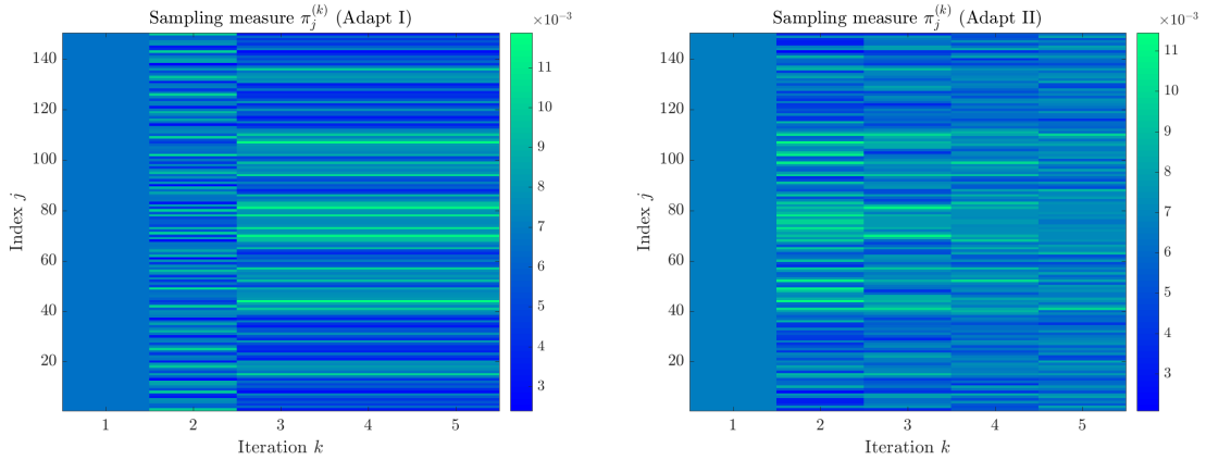
Figure 7: Evolution of the sampling measure \pi_j^{(k)} as a function of the iteration k for adaptive strategies (Adapt I) and (Adapt II).
