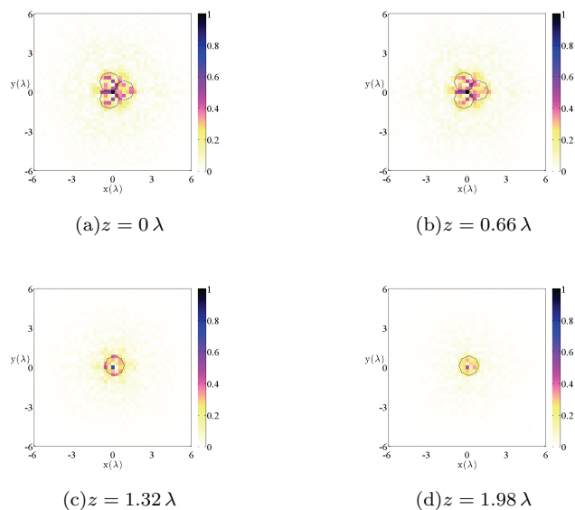
Fig. 7. Maps reconstructed at several altitudes using the pyramid of spheres scattered fields in the S_{\theta\theta} polarization. The real spheres boundaries are plotted in black.
