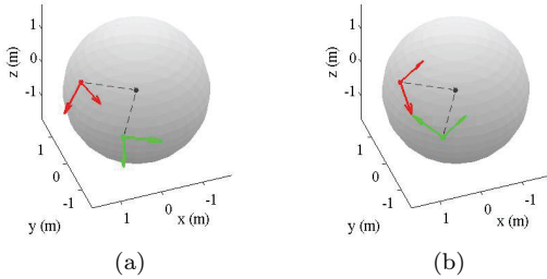
Fig. 3. For a given couple of transmitter and receiver positions (source : (r^T = 102\lambda, \theta^T = 100^\circ, \phi^T = 60^\circ) , receiver (r^R = 102\lambda, \theta^R = 150^\circ, \phi^R = 90^\circ) ), representation of the basis vectors for the source (red) and for the receiver (green) (the \mathbf{k}_i and \mathbf{k}_s vectors are plotted in black (- -)) under (a) the spherical convention, (b) the Bohren and Huffman convention.
