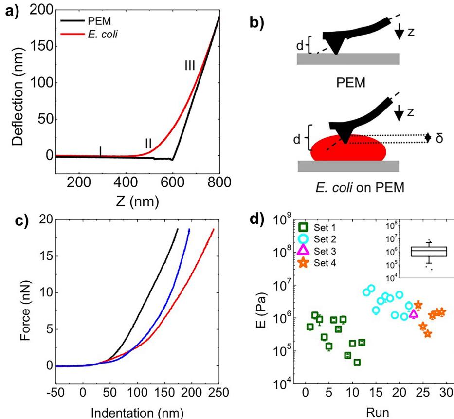
Fig. 2. (a) Raw FCs in approach (deflection as a function of the displacement z ) on a bacterium and the PEM substrate. (b) Schemes of the tip behavior when interacting with a solid substrate and a soft sample, showing several parameters: d , the cantilever deflection, z the displacement and \delta the indentation (as stated in Materials and Methods section). (c) FCs in approach (after treatment by the Matlab routine) for different bacteria of the same experimental set. (d) Young modulus E of E. coli cells, from independent experimental sets of bacteria (one point stands for one bacterium, i.e. one FC). A box chart is shown in inset to visualize the dispersion of E according to different percentiles.
