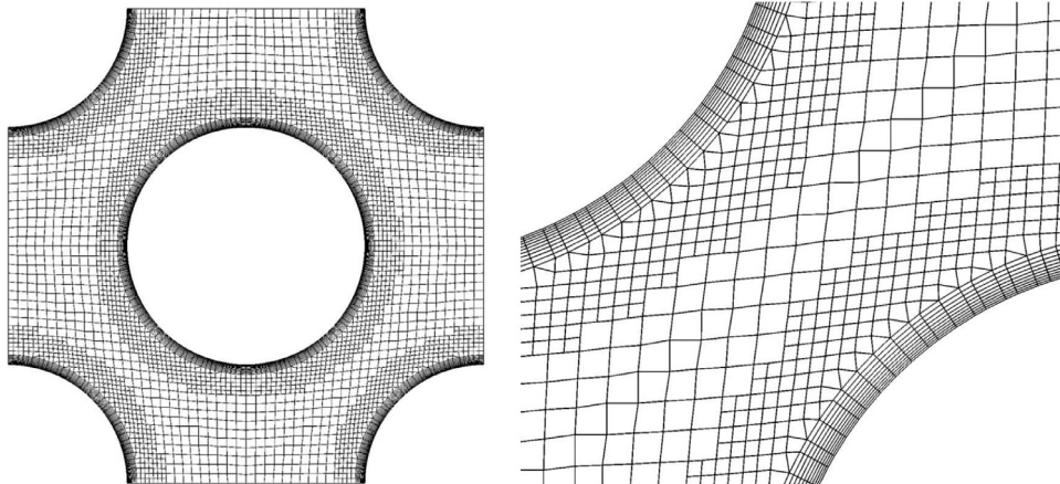
Fig. A.17. Mesh used for the computation; top view (left) and zoom in the boundary layer region (right). \epsilon = 0.6 .
