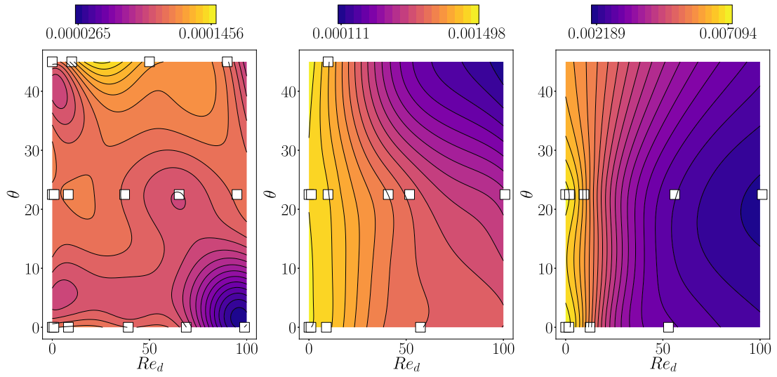
Fig. 13. Response surfaces of H_{11} with \phi = 0^\circ for porosity \epsilon = 0.4, 0.6, 0.8 , from left to right.
