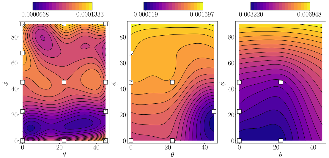
Fig. 15. Response surfaces of H_{11} with Re_d = 40 for porosity \epsilon = 0.4, 0.6, 0.8 , from left to right.
