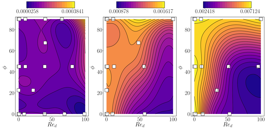
Fig. 14. Response surfaces of H_{11} with \theta = 0^\circ for porosity \epsilon = 0.4, 0.6, 0.8 , from left to right.
