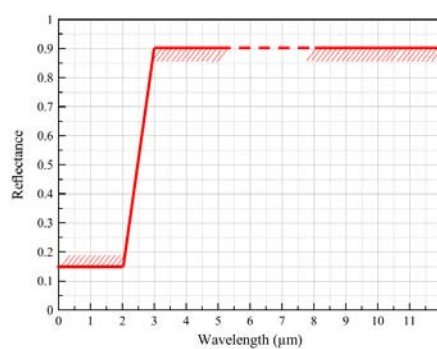
Fig. 1. Optical specifications of the optical filter. Low reflectivity has to be achieved from visible up to 2.5 \mu\text{m} and a mirror-like behavior from 3 to 12 \mu\text{m} .
