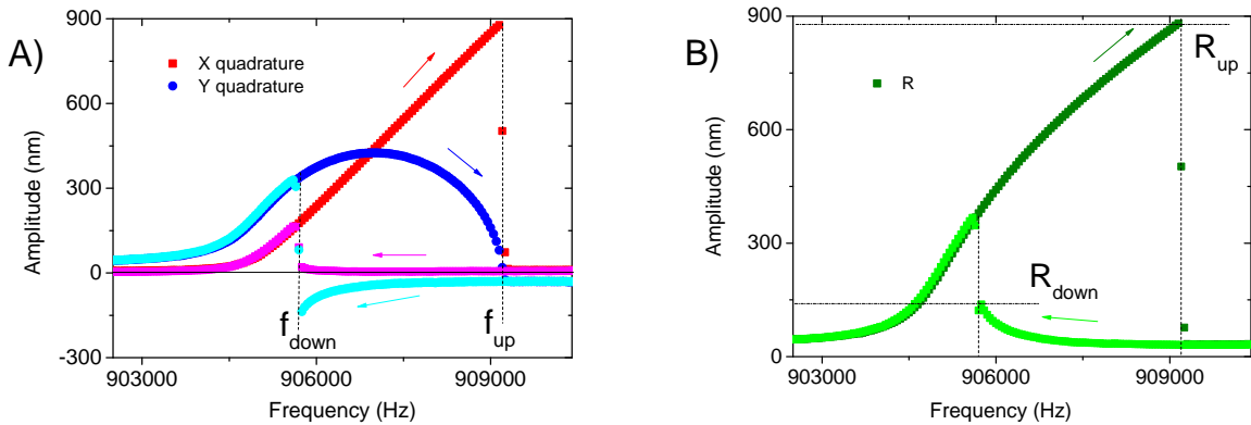
Figure 2: Nonlinear (Duffing) resonance. A) Duffing resonance line (X and Y quadratures) measured on the 250 \mu\text{m} device at 4.2 K in vacuum, for a drive force of 81 pN, in a 1 T field. The directions of frequency sweeps are depicted by arrows. Vertical dashed lines indicate the two bifurcation points f_{\text{up,down}} . B) Amplitude R = \sqrt{X^2 + Y^2} corresponding to A). Bifurcation points are indicated with their amplitudes R_{\text{up,down}} .
