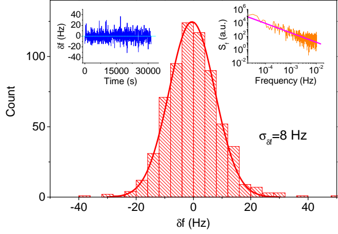
Figure 5: Large amplitude statistics. Similar graphs as in Fig. 4 obtained on the upper bifurcation point f_{up} (frequency jumps time-trace in the left inset, power spectrum of frequency in the right inset and histogram of \delta f in the main of the graph). The line is a Gaussian fit, while the power spectrum follows 1/f^{1.4} (see text).
