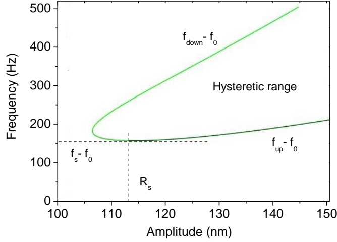
Figure 3: Bifurcation branches. Calculated bifurcation frequencies from Eqs. (1-2) for the 250 \mu\text{m} device and magnetomotively-loaded Q of 5000 (1 T field).
