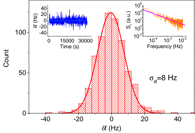
Figure 5: Large amplitude statistics. Similar graphs as in Fig. 4 obtained on the upper bifurcation point f_{up} (frequency jumps time-trace in the left inset, power spectrum of frequency in the right inset and histogram of \delta f in the main of the graph). The line is a Gaussian fit, while the power spectrum follows 1/f^{1.4} (see text).
