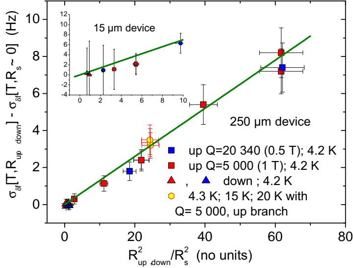
Figure 6: Universal plot for mode 1. Frequency noise increase vs squared amplitude normalized to the spinodal value R_s , for the first mode n = 1 of the 250 \mu\text{m} device. Various T_0 and B_0 (hence Q ) have been used (see legend). Squares stand for upper branch bifurcation, triangles for lower. Inset: same result obtained with a 15 \mu\text{m} beam having \beta = 1.1 \times 10^{19} \text{ Hz/m}^2 (4.2 K and Q = 17\,000 red squares; 800 mK and Q = 31\,000 blue dots; the magnetomotive field broadening was negligible). The green line is a linear fit (see text).
