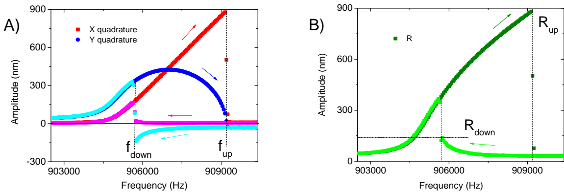
Figure 2: Nonlinear (Duffing) resonance. A) Duffing resonance line (X and Y quadratures) measured on the 250 \mu\text{m} device at 4.2 K in vacuum, for a drive force of 81 pN, in a 1 T field. The directions of frequency sweeps are depicted by arrows. Vertical dashed lines indicate the two bifurcation points f_{\text{up,down}} . B) Amplitude R = \sqrt{X^2 + Y^2} corresponding to A). Bifurcation points are indicated with their amplitudes R_{\text{up,down}} .
