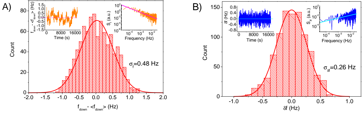
Figure 4: Statistics on frequency at low amplitudes. A): histogram obtained on the f_{\text{down}} relaxation point of Fig. 2 (left inset: actual frequency time-trace; right inset: power spectrum of the frequency fluctuations, displaying 1/f -type structure). B): histogram obtained on the frequency jumps \delta f computed from the f_{\text{down}} time-trace (left inset: \delta f time-trace; right inset: power spectrum). The lines are Gaussian fits, and the power-law dependencies of the spectra are discussed in the text.
