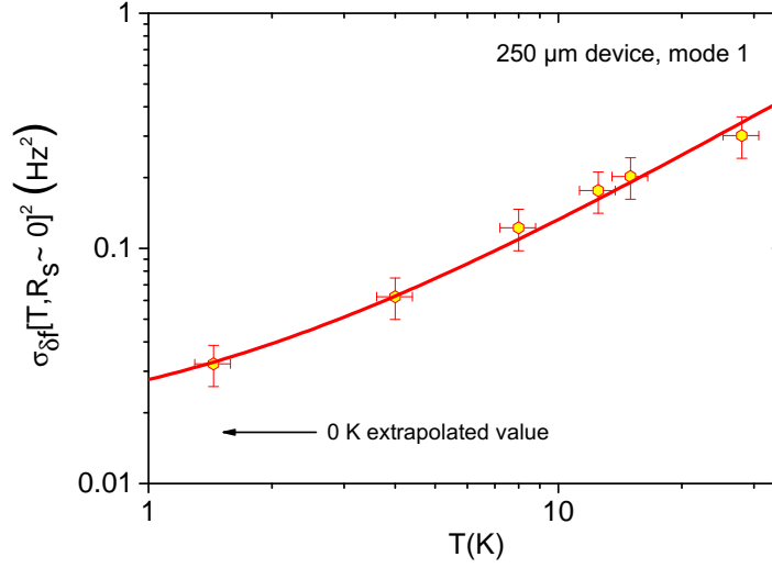
Figure 8: Temperature dependence of frequency fluctuations. Allan variance \sigma_{\delta f}^2 as a function of temperature (first mode of 250 \mu\text{m} device), as obtained for small motion R \rightarrow R_s \sim 0 . The line is a linear fit, with the T_0 = 0 K extrapolated value emphasized by the arrow (see text). The variance of damping fluctuations \sigma_{\delta \Delta f}^2 is constant in the same range of temperatures.
