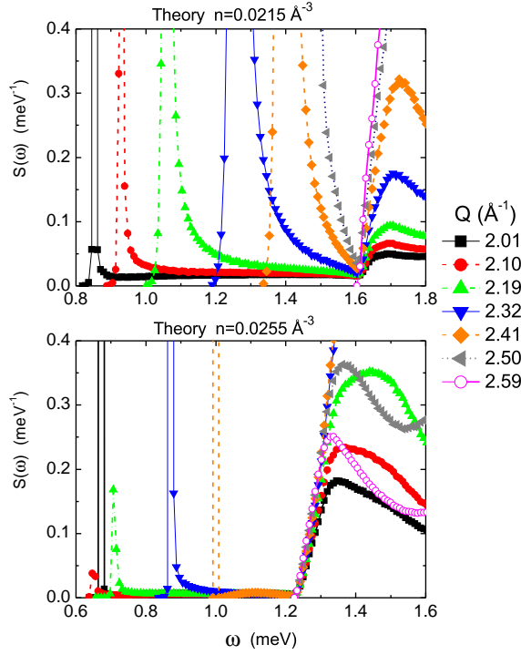
FIG. 13. S(Q, \omega) calculated for wave vectors in the region of the ghost-roton, at densities n = 0.0215 and 0.0255 \text{ \AA}^{-3} , associated to P = 0 and P = 24 bars respectively.
