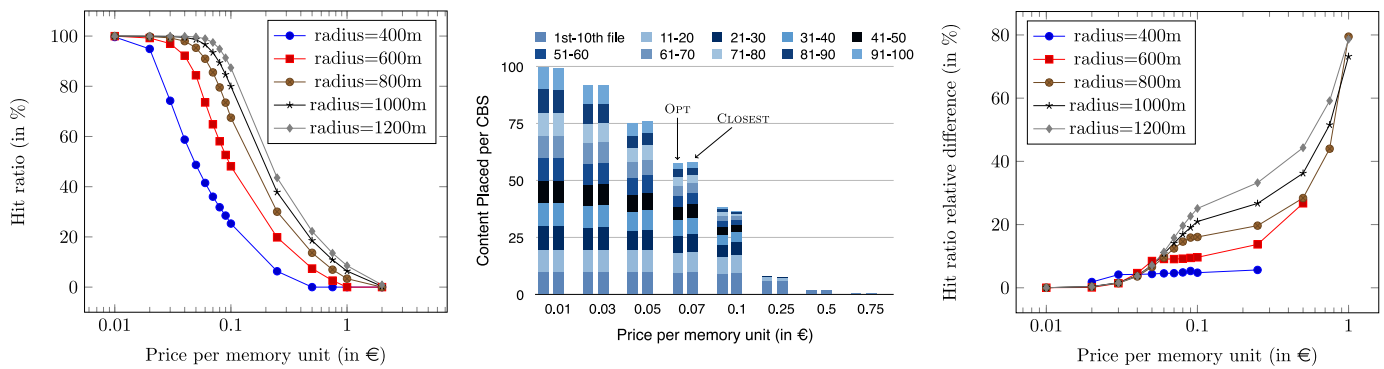
Fig. 5: Linear savings function. (a): Hit ratio in relation to price for different coverage radii with OPT association. (b): Cache lease and placement of popular files depending on cache unit price. Each left column represents the case of OPT association, each right column with CLOSEST association. (c): Relative difference between the hit ratio achieved by OPT to CLOSEST over cache unit price for different coverage radii.
