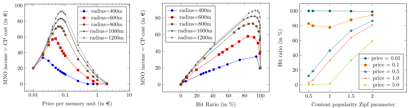
Fig. 6: Linear savings function. (a): Income of MNO in relation to price per cache unit for different coverage radii with OPT. (b): MNO income/CP investment over hit ratio for different coverage radii with OPT: Achieving the hit ratio on the x-axis results in the MNO income on y-axis. (c): Hit ratio in relation to Zipf parameter for different prices with OPT.
