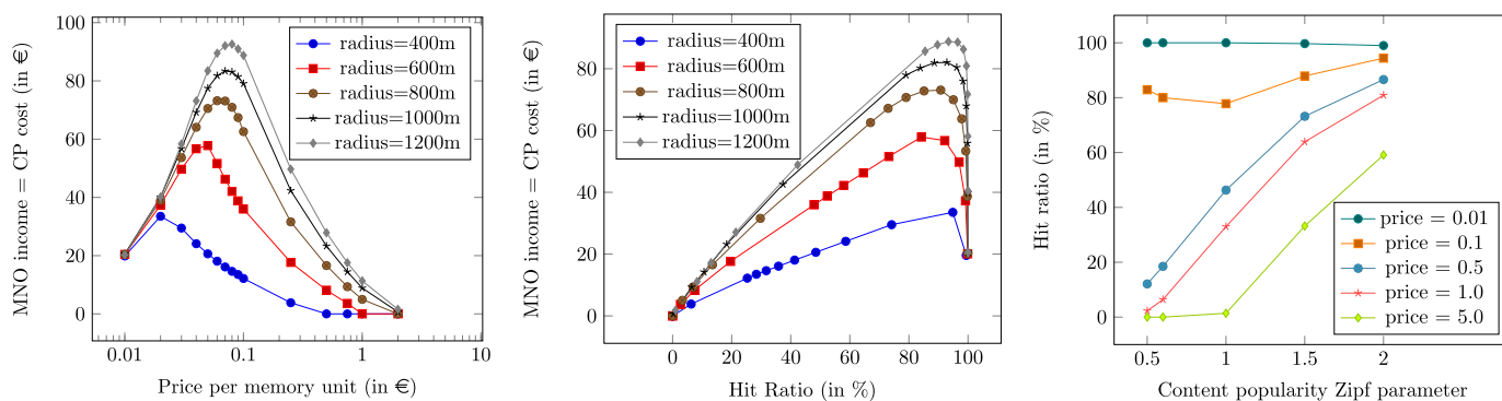
Fig. 6: Linear savings function. (a): Income of MNO in relation to price per cache unit for different coverage radii with OPT. (b): MNO income/CP investment over hit ratio for different coverage radii with OPT: Achieving the hit ratio on the x-axis results in the MNO income on y-axis. (c): Hit ratio in relation to Zipf parameter for different prices with OPT.
