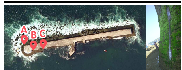
Figure 2. Left: Artha breakwater (A. pressure sensors, B. data acquisition system, C. photovoltaic panel and data transmitter unit). Right: photograph of the 2 pressure sensors embedded in the wall structure.
