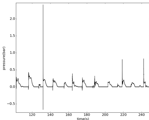
Figure 5. Illustration of short and intense impacts.
