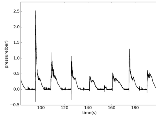
Figure 6. Illustration of slower impacts.
