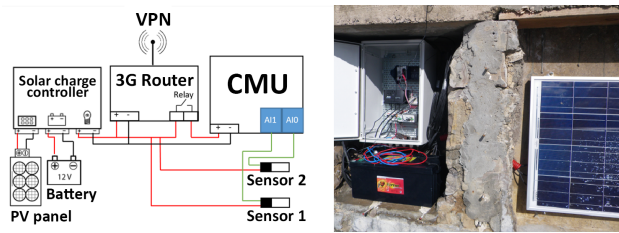
Figure 3. Installation setup on the breakwater. Left: Block-diagram. Right: Photograph.
