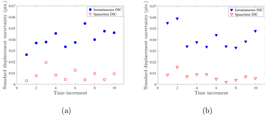
Figure 14: Standard deviations on (a) horizontal and (b) vertical displacements for instantaneous and spacetime DIC procedures for the calibration phase
