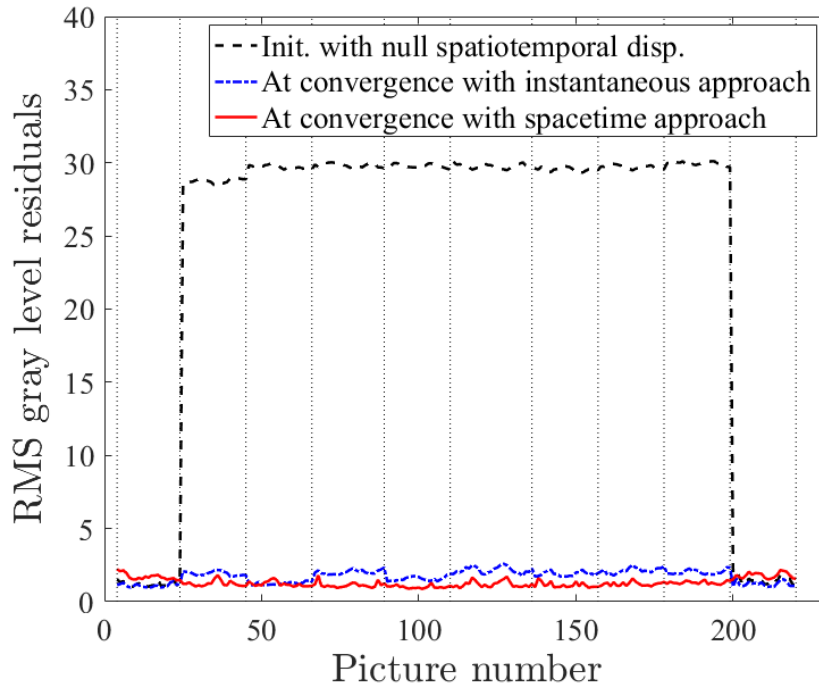
Figure 12: Root mean square gray level residuals for all analyzed pictures for instantaneous DIC (blue line), spacetime DIC (red line). The black line corresponds to the RMS gray level residuals of the raw picture difference ( i.e. , with null displacements). The dotted vertical lines depict the time increments.
