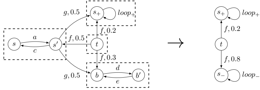
Figure 1: Min-reduction of an MDP
