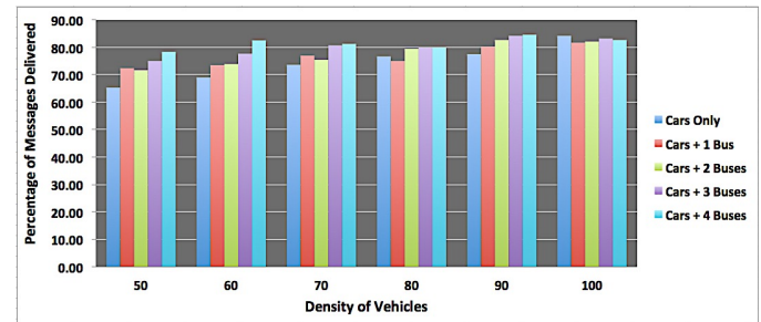
FIGURE I. THE EFFECT OF BUSES ON THE PERCENTAGE OF MESSAGES DELIVERED USING MAXPROP
