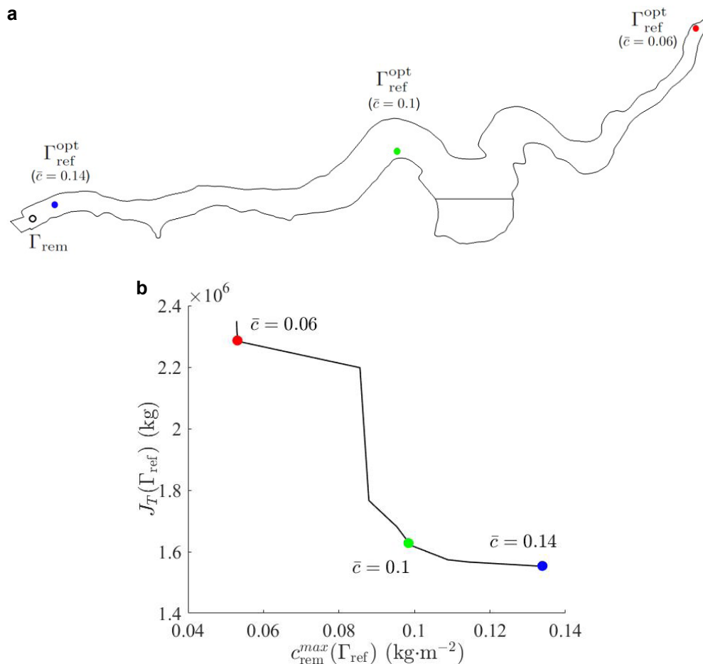
Figure 5. Graphical interpretation of the optimization results solution of equation 2 when \bar{c} \in \{0.06, 0.1, 0.14\} kg \cdot m^{-2} : a) optimal refilling locations \Gamma_{ref}^{opt} , b) objective values J_T(\Gamma_{ref}^{opt}), c_{rem}^{max}(\Gamma_{ref}^{opt}) associated to these optimal refilling locations. The black curve represents the Pareto front.
