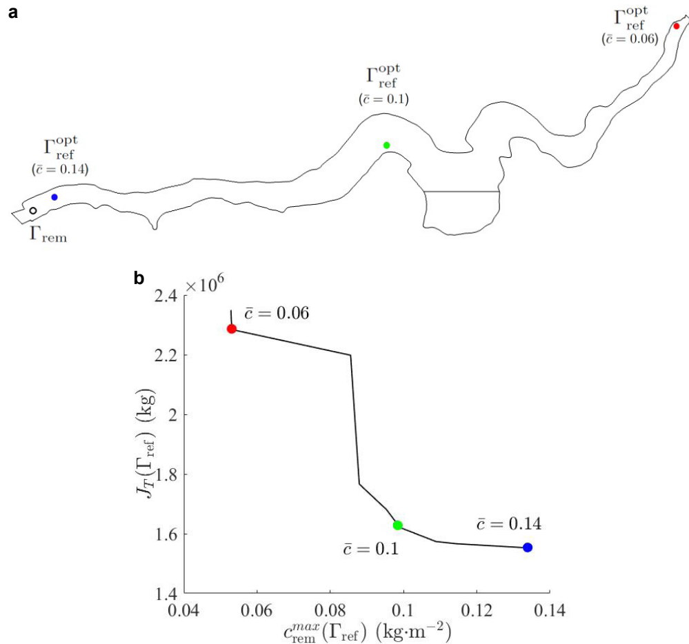
Figure 5. Graphical interpretation of the optimization results solution of equation 2 when \bar{c} \in \{0.06, 0.1, 0.14\} kg·m -2 : a) optimal refilling locations \Gamma_{ref}^{opt} , b) objective values J_T(\Gamma_{ref}^{opt}), c_{rem}^{max}(\Gamma_{ref}^{opt}) associated to these optimal refilling locations. The black curve represents the Pareto front.
