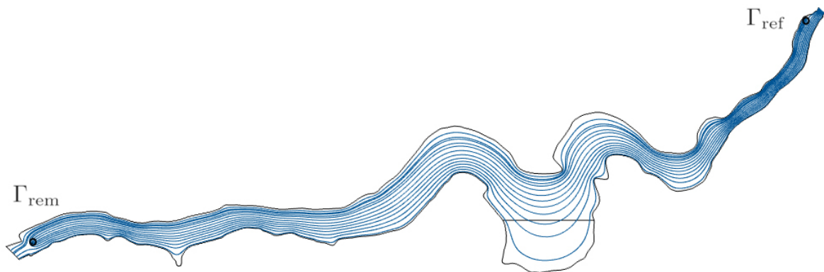
(a) Water current streamlines associated to a specific choice of \Gamma_{ref} and \Gamma_{rem} .
